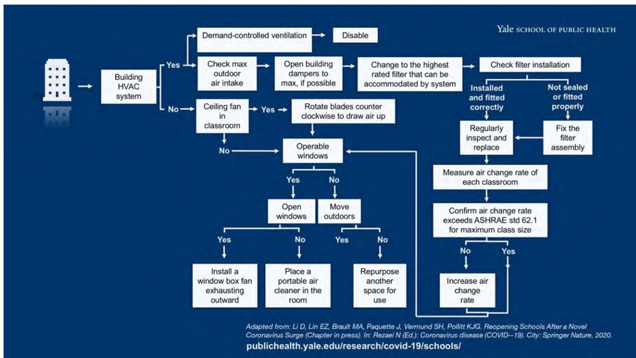
Figure 3: Simplified flow chart for HVAC and building control measures from https://publichealth.yale.edu/research/covid-19/schools/ventilation/ .
