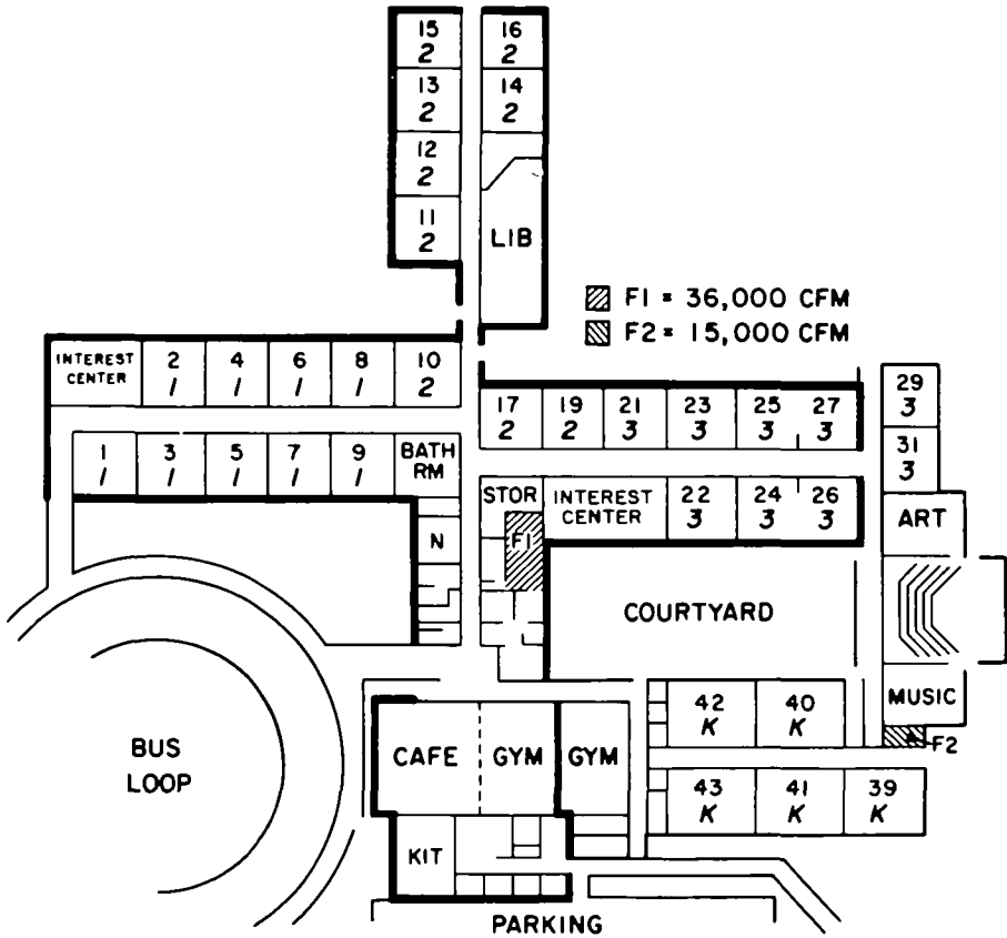
FIGURE 2. Floor plan of an upstate New York elementary school which experienced a measles epidemic in spring, 1974. The main building, constructed in 1961, is outlined in bold lines. F1 identifies the fan room servicing these rooms (36,000 cfm = 1019.4 m 3 /min). The 1971 addition appears to the right and below the courtyard. F-2 identifies its fan room (15,000 cfm = 424.8 m 3 /min). Within the floor area of each room, the room number appears above and the grade below.
