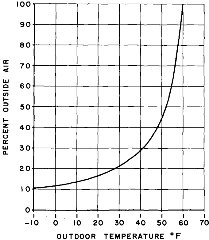
FIGURE 3. Response of the two ventilating systems to changes in outdoor temperature at an upstate New York elementary school which experienced a measles epidemic in spring, 1974. The percentage of recirculated air = 100 minus per cent outside air. This curve is specific for room temperature of 68 F (19 C). For conversion to C: -10 F = -23.3 C; 0 F = -17.8 C; 10 F = -12.2 C; 20 F = -6.7 C; 30 F = -1.1 C; 40 F = 4.4 C; 50 F = 10 C; 60 F = 15.6 C; 70 F = 21.1 C.
